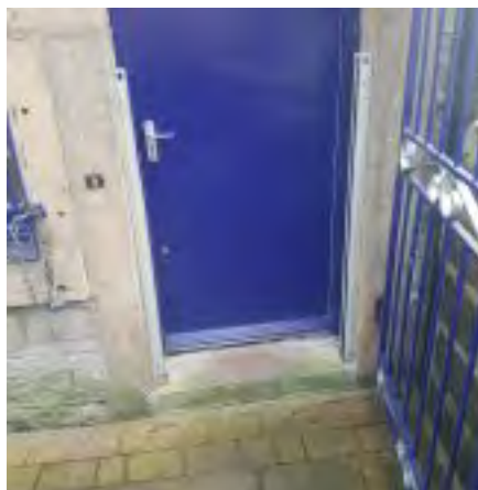
Flood barriers to all doors.
