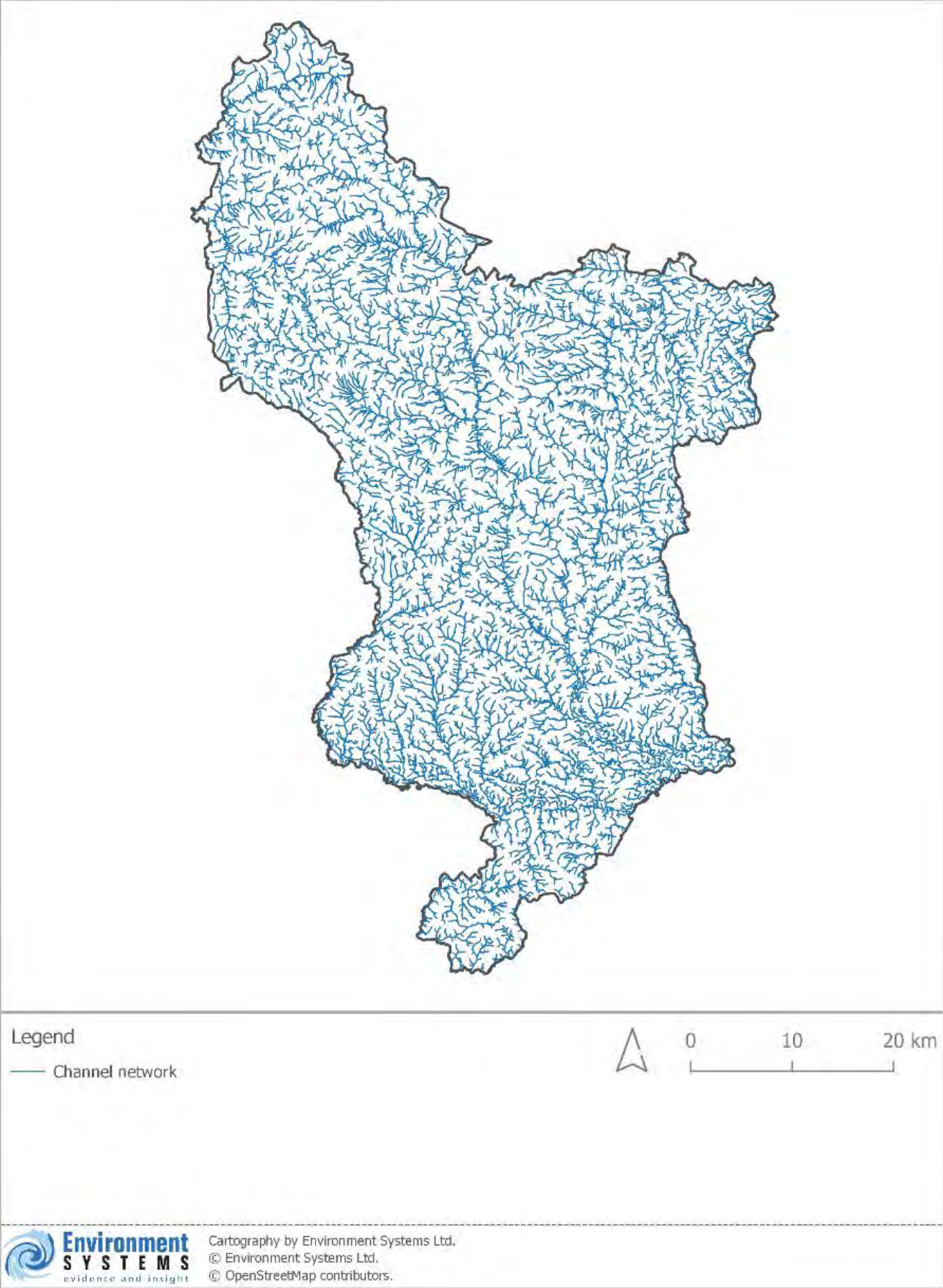
Figure 32: Channel Network
