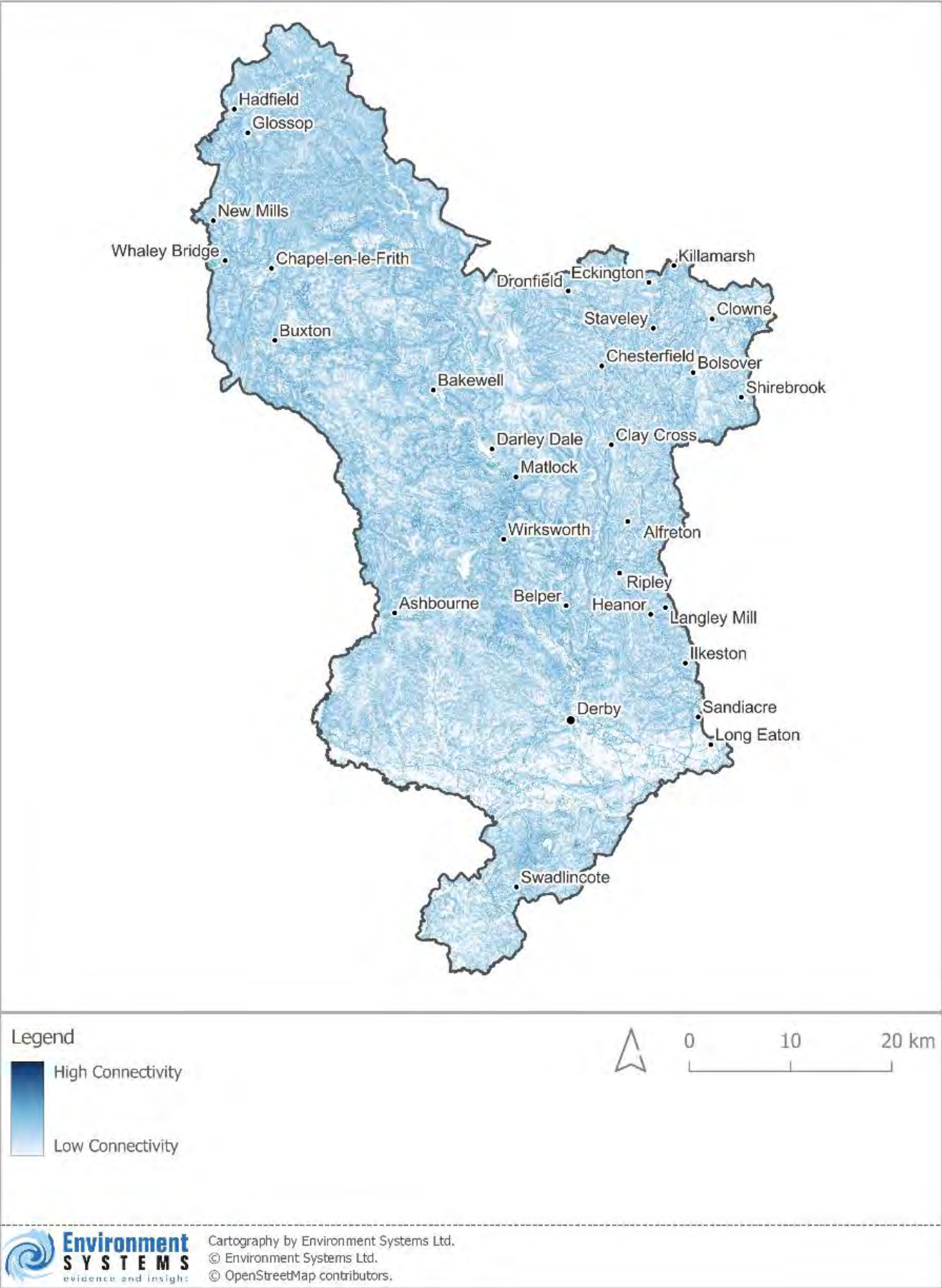
Figure 33: Hydrological connectivity
