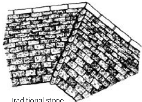
Traditional stone valley detail showing pointed valley slates
