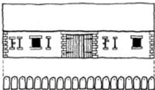
Measurement of the building, to ensure that the largest slates are sufficient to form the eaves course.
